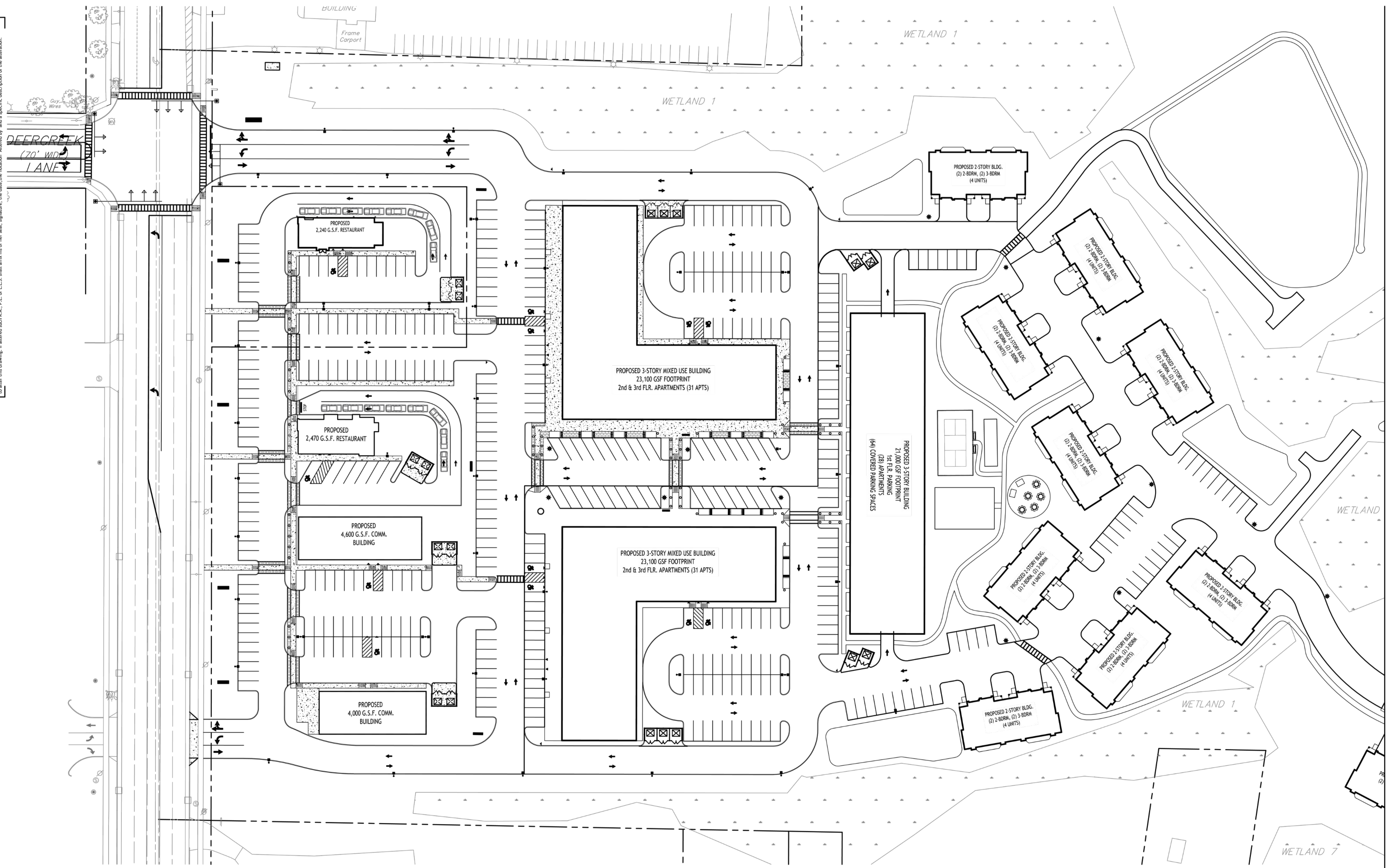
N Site Plan SCALE: 1"=40'
